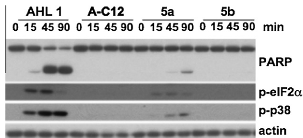
Figure 2. Biological activities of AHL 1 , C 12 -HSL (A-C12; negative control) and its alkynyl analogs 5a and 5b in mammalian cells. BMDM were treated as indicated, and cellular extracts were analyzed by Western blot for the cleavage of PARP, phosphorylated forms of eIF2α (p-eIF2α) or p38 (p-p38) and actin as a loading control.
