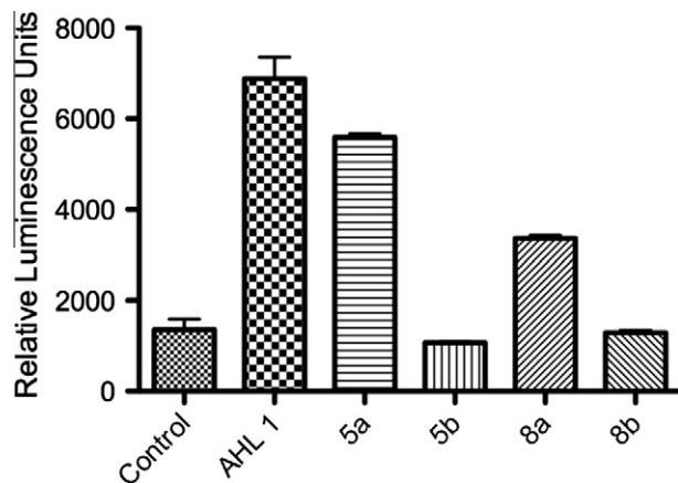
Figure 4. Autoinducer activities of alkynyl- and azido-AHL analogs in P. aeruginosa . Relative luminescence units were normalized with respect to cell viability ( OD_{600} ).
