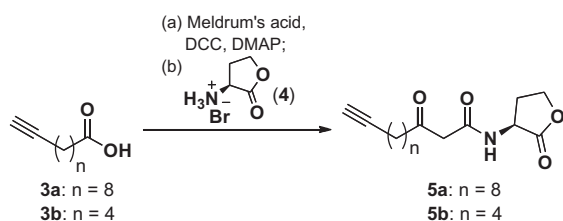
Scheme 1. Synthesis of alkynyl AHL analogs.
