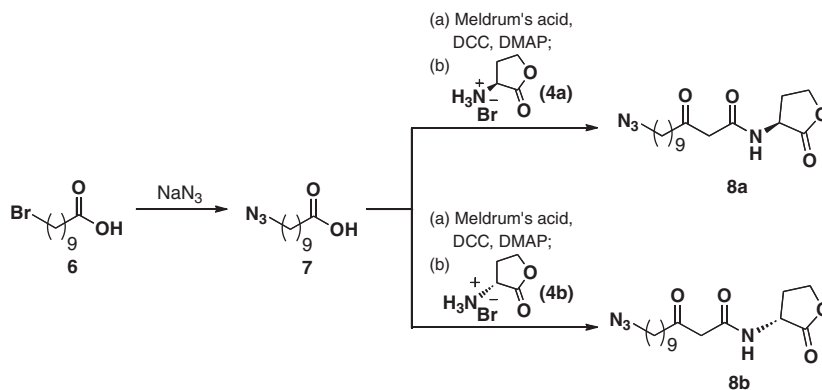
Scheme 2. Synthesis of azido AHL analogs.
