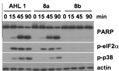
Figure 3. Biological activities of azido analogs 8a and 8b in mammalian cells.
